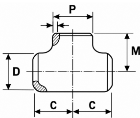
REDUCING TEES
