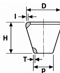
CONCENTRIC REDUCERS
