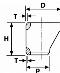
ECCENTRIC REDUCERS
