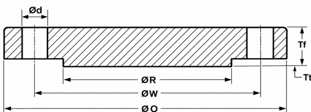
BLIND FLANGE
