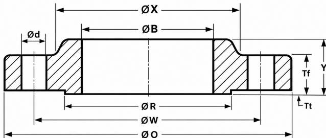
SLIP-ON FLANGE
