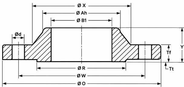
WELDING NECK FLANGE
